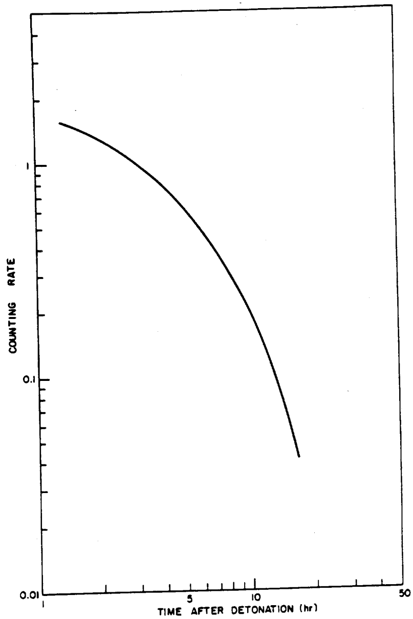
Figure 3.7 Sticky-pan decay curve.
