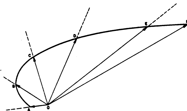
Figure 1.7 Example of a hodograph.
