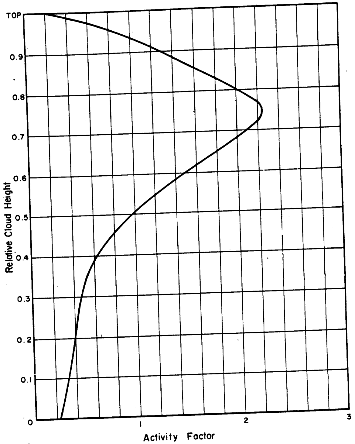
Figure 1.1 Hardtack model space distribution. For a uniform distribution of activity with height activity, the factor would equal 1 for all heights.
