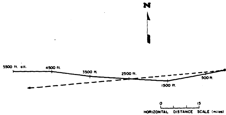
Figure 1.4 Hodograph of wind structure assumed for model calculations. Calculations were made along dashed line. Hodograph is drawn for 1,000-foot-per-hour balloon-rise rate.
