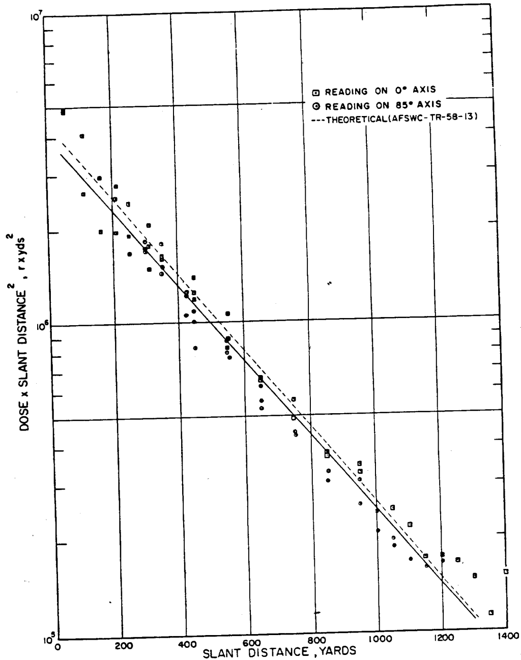
Figure 3.5 Summary of initial gamma, RD^2 versus D .
