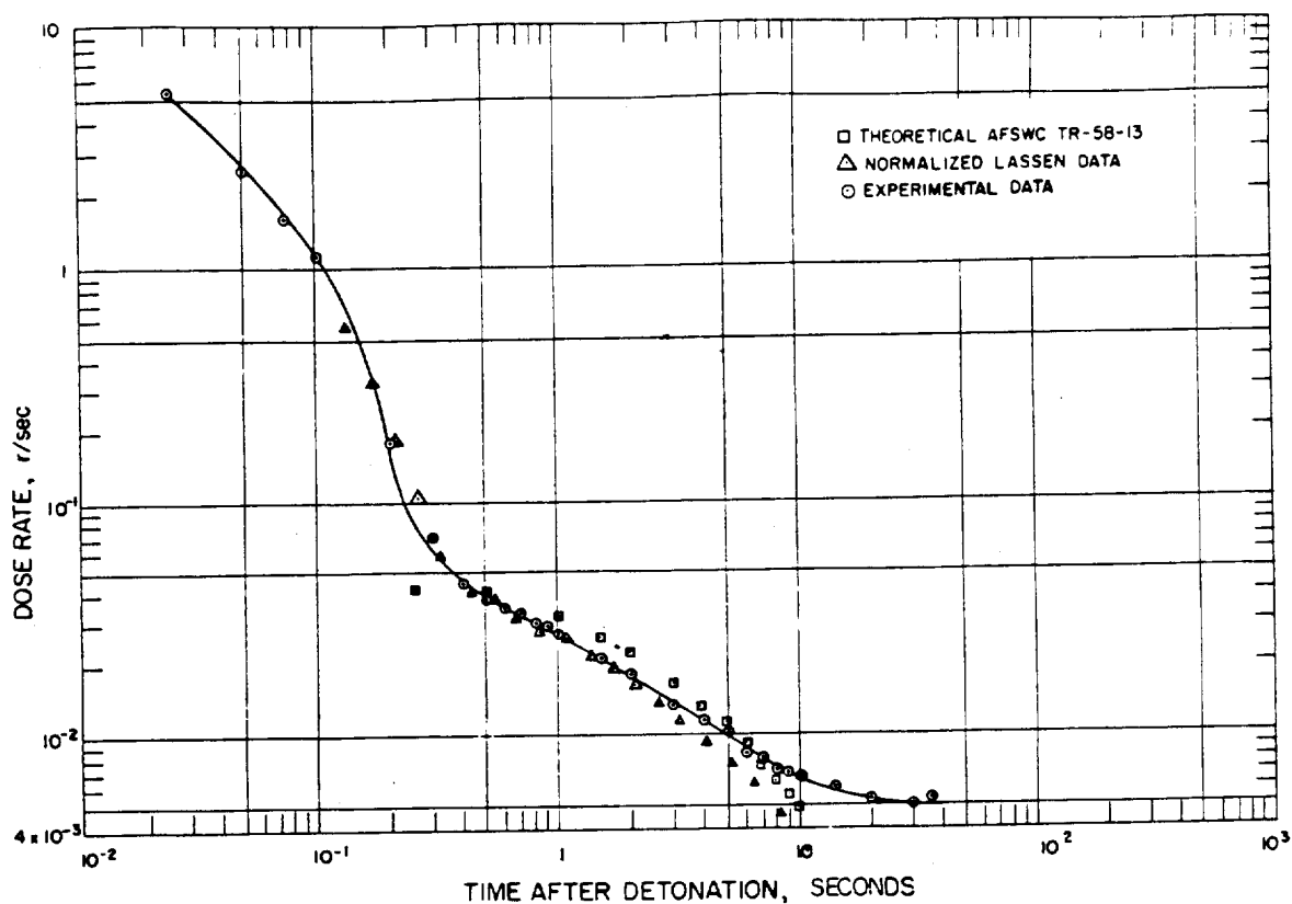
Figure 3.1 Initial-gamma dose rate versus time at 750 yards, 85-degree axis.
