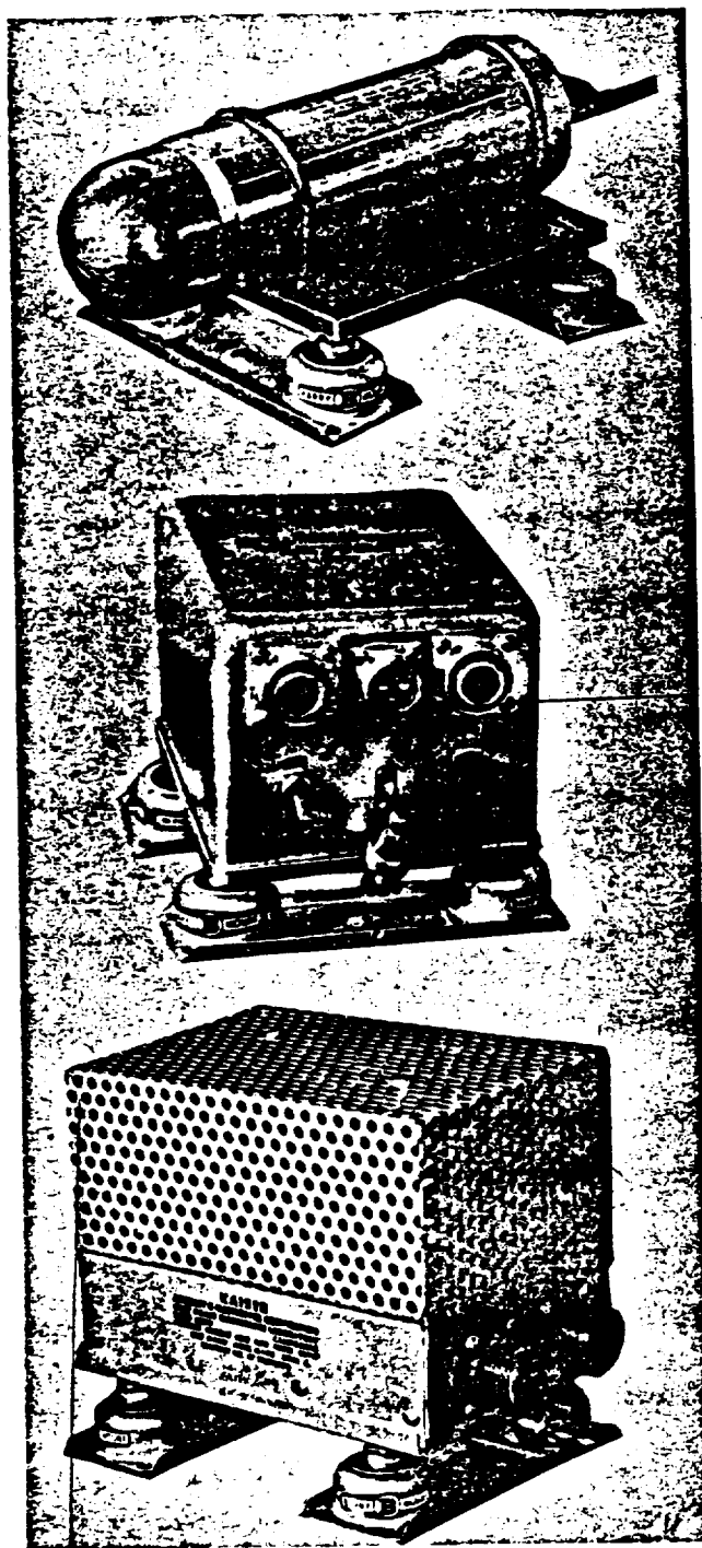
Figure 2.4 Kaiser dose-rate instrument, showing probe, compressor-oscillator-amplifier unit, and power supply (top to bottom).
