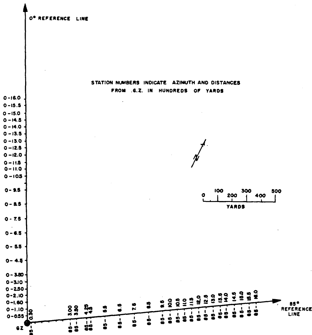
Figure 2.3 Station plot plan.
