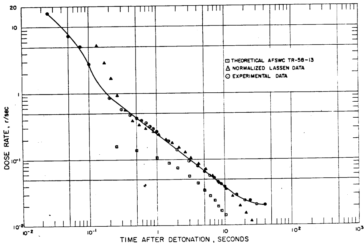
Figure 3.2 Initial-gamma dose rate versus time at 550 yards, 85-degree axis.
