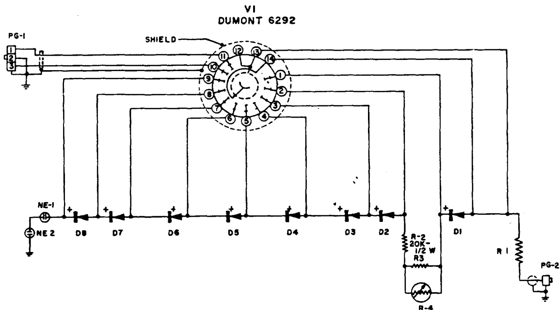
Figure 2.6 Kaiser dose-rate instrument, gamma scintillation probe.
