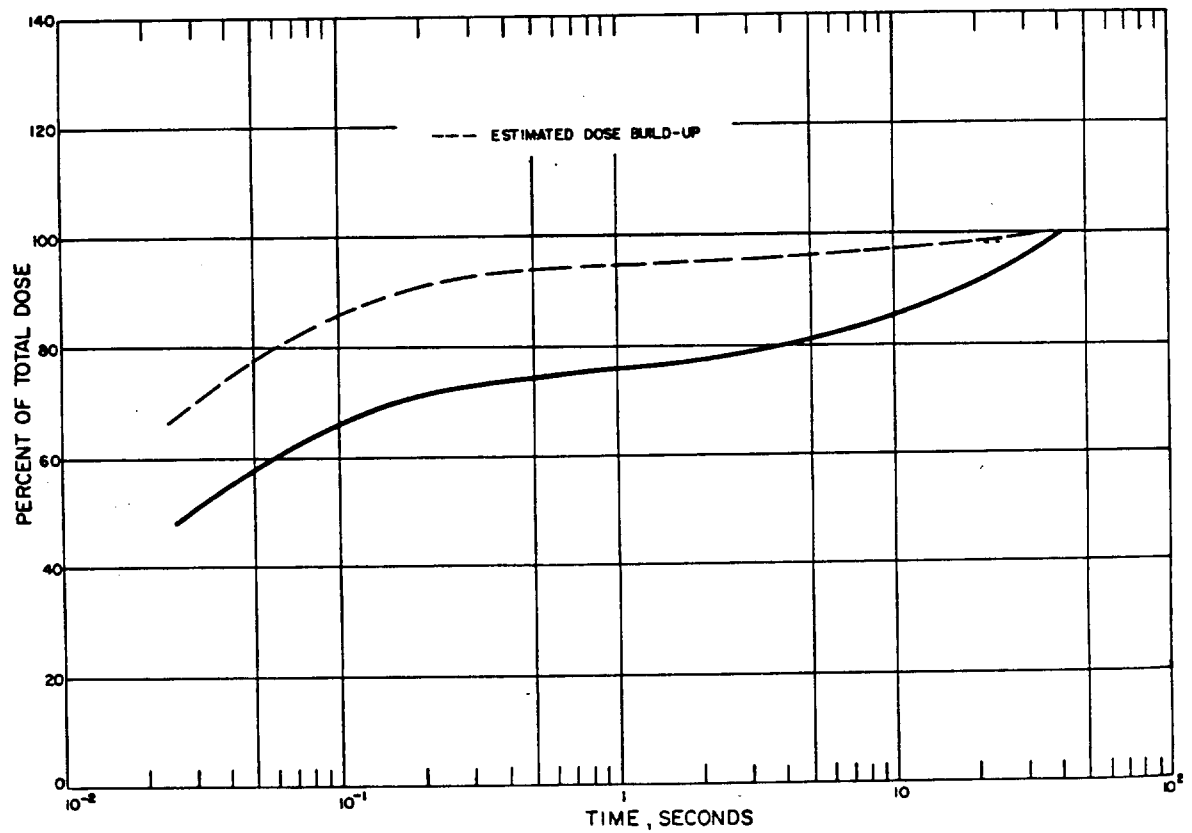
Figure 3.4 Integrated initial-gamma dose percent of total dose versus time, 750 yards.
