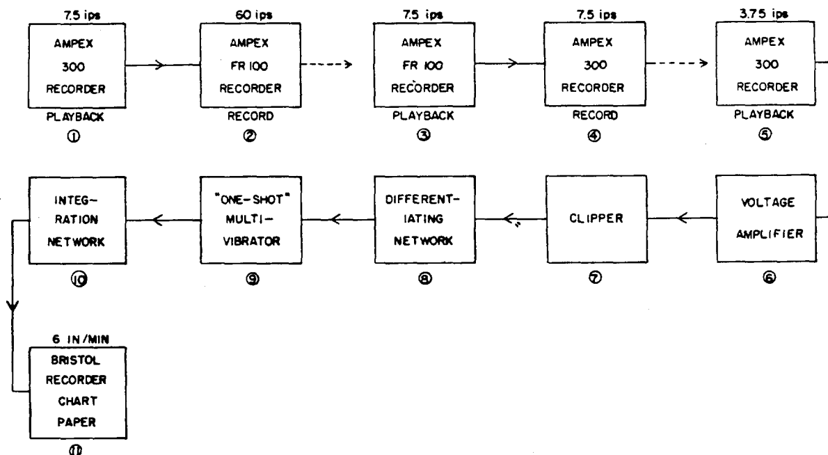
Figure 2.10 Block diagram of Kaiser playback-and-readout equipment.
