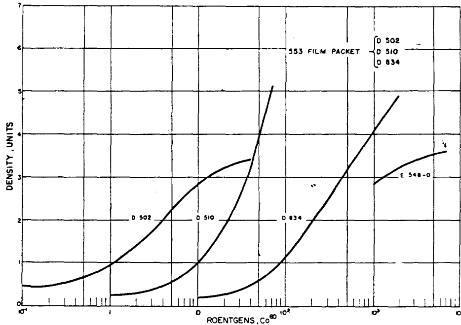
Figure 2.12 Calibration curves for NBS dosimeter film.
