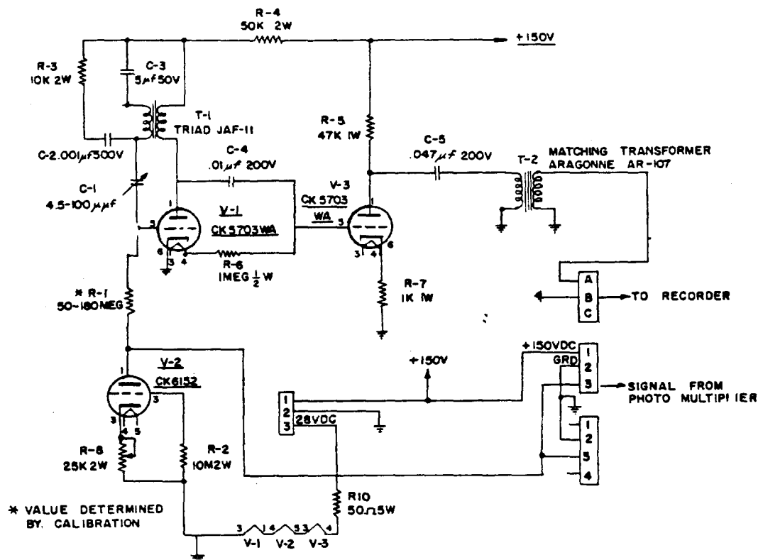
Figure 2.7 Kaiser dose-rate instrument, oscillator and compression circuit.
