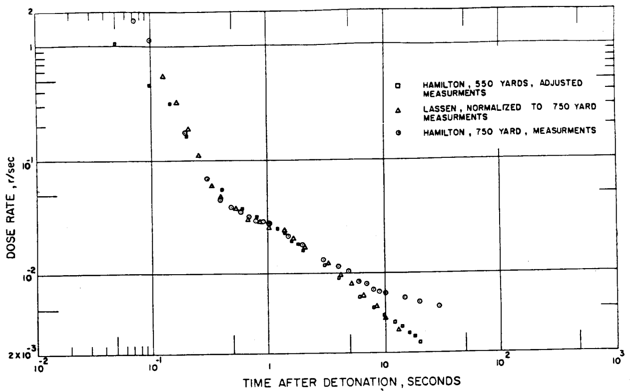
Figure 3.3 Summary of dose-rate data.
