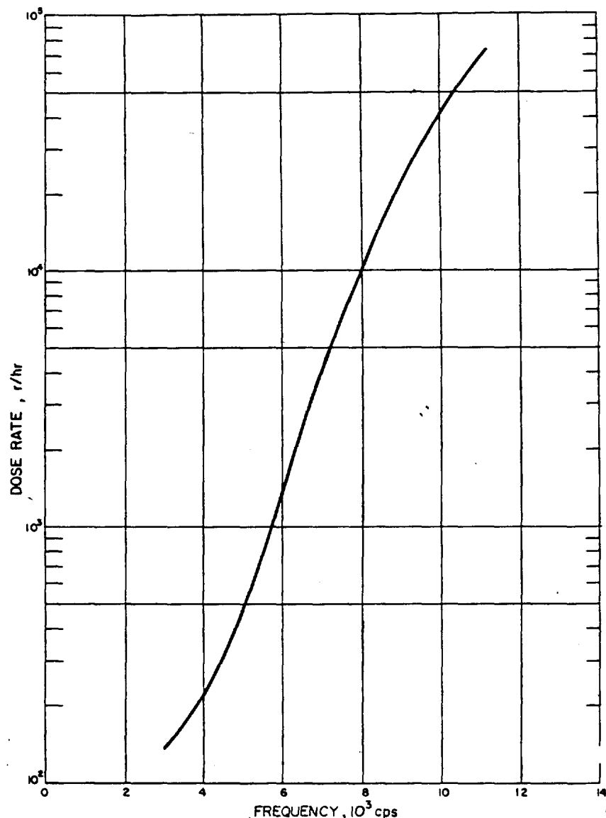
Figure 2.9 Calibration curve for Kaiser dose-rate instrument, 750-yard station.
