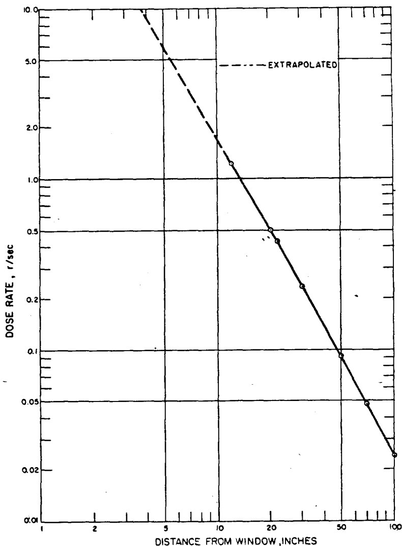
Figure 2.11 Calibration curve for 500-curie \text{Co}^{60} source.
