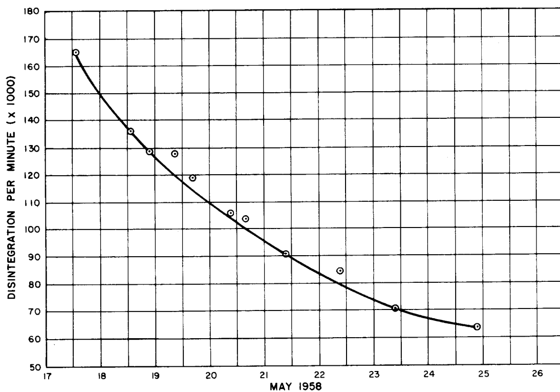
Figure 5.2 Fallout Tray Sample Decay Curve
