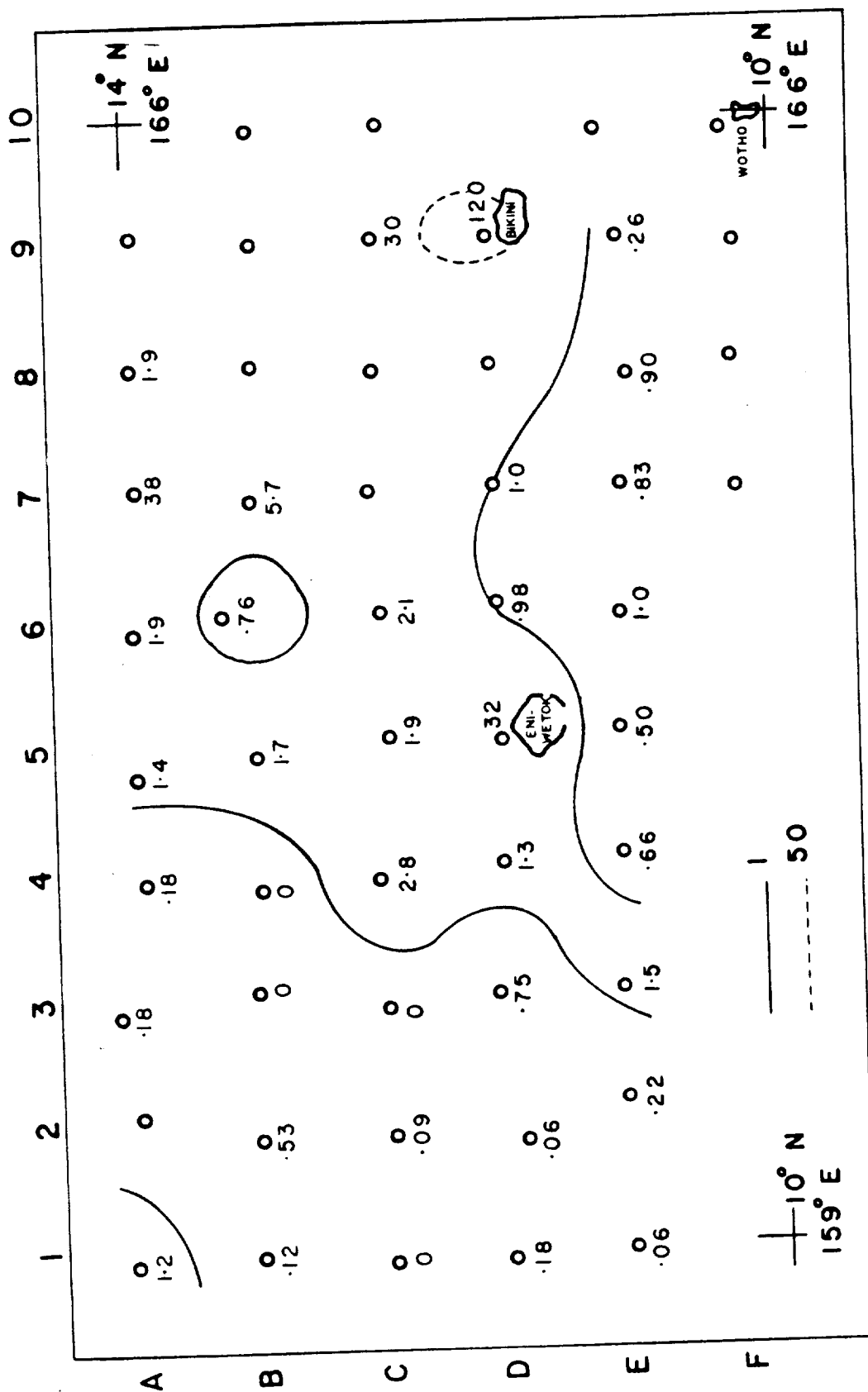
FIG. 15. RADIOACTIVITY OF WATER FROM 75 METER DEPTH IN THOUSANDS OF DISINTEGRATIONS PER MINUTE PER LITER.
