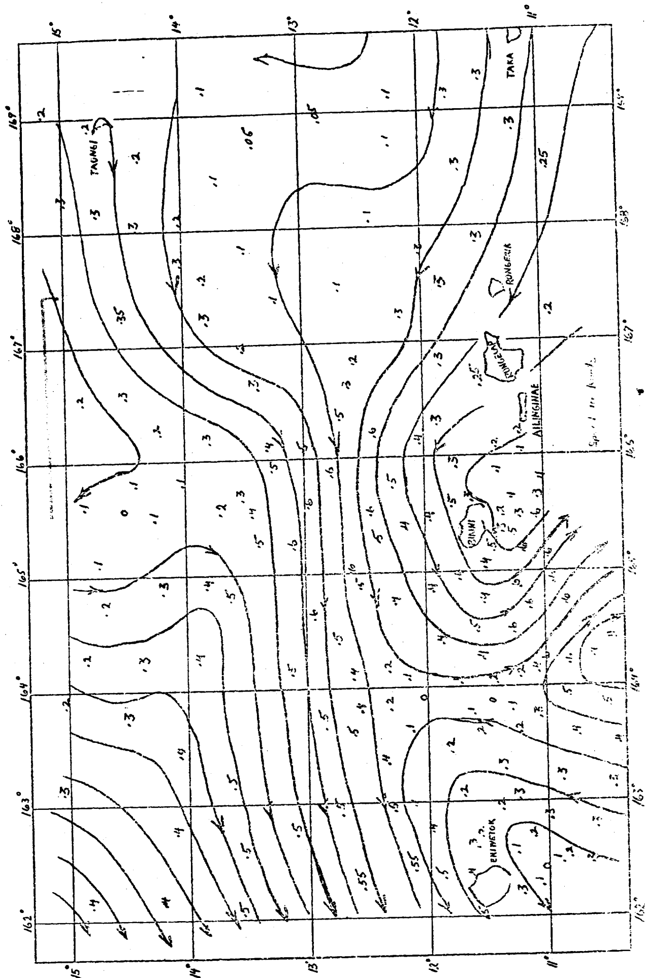
DIRECTION AND SPEED OF SURFACE CURRENTS
