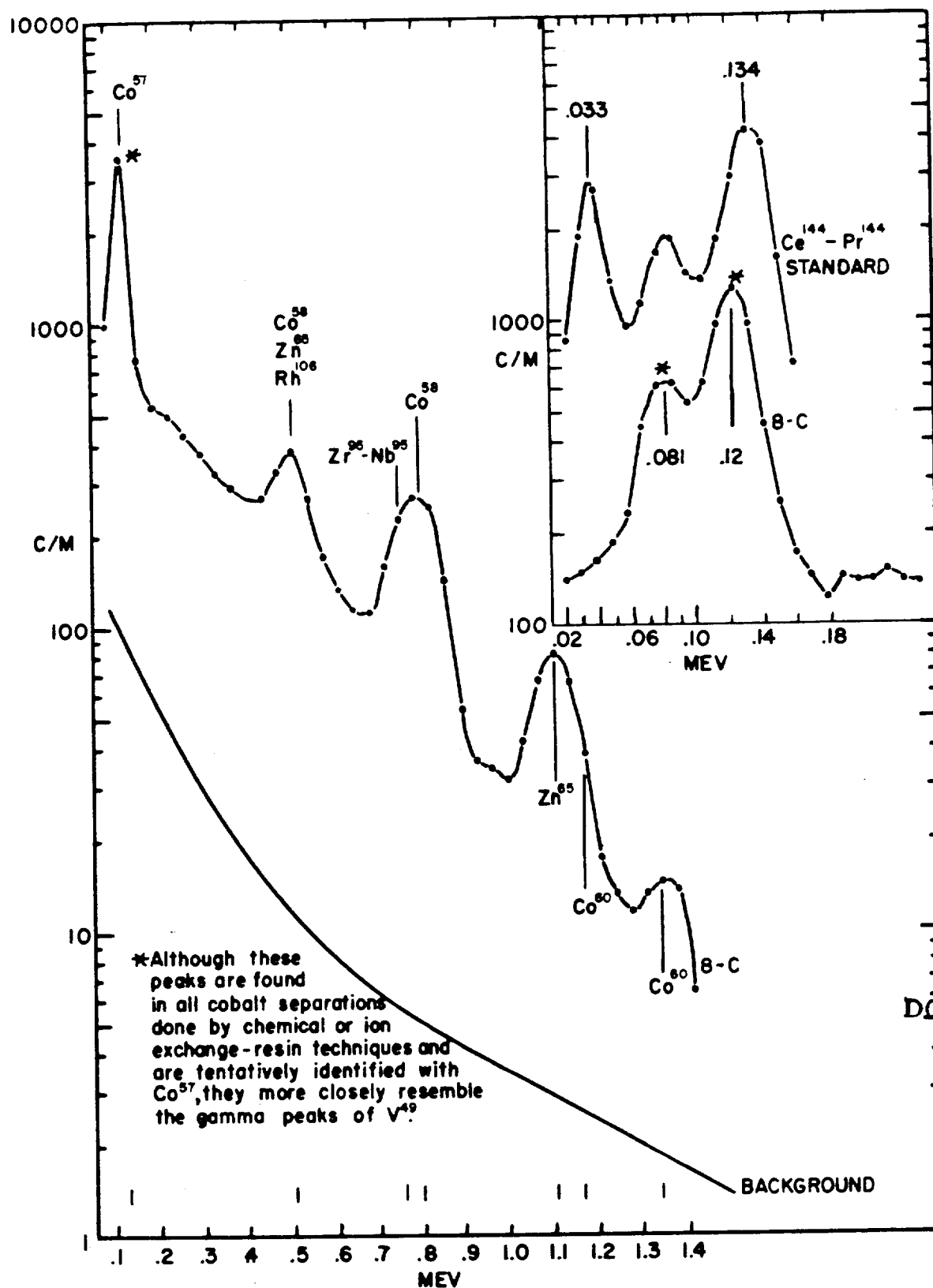
Fig. 10. Gamma spectrum of Walton plankton sample B-C.
