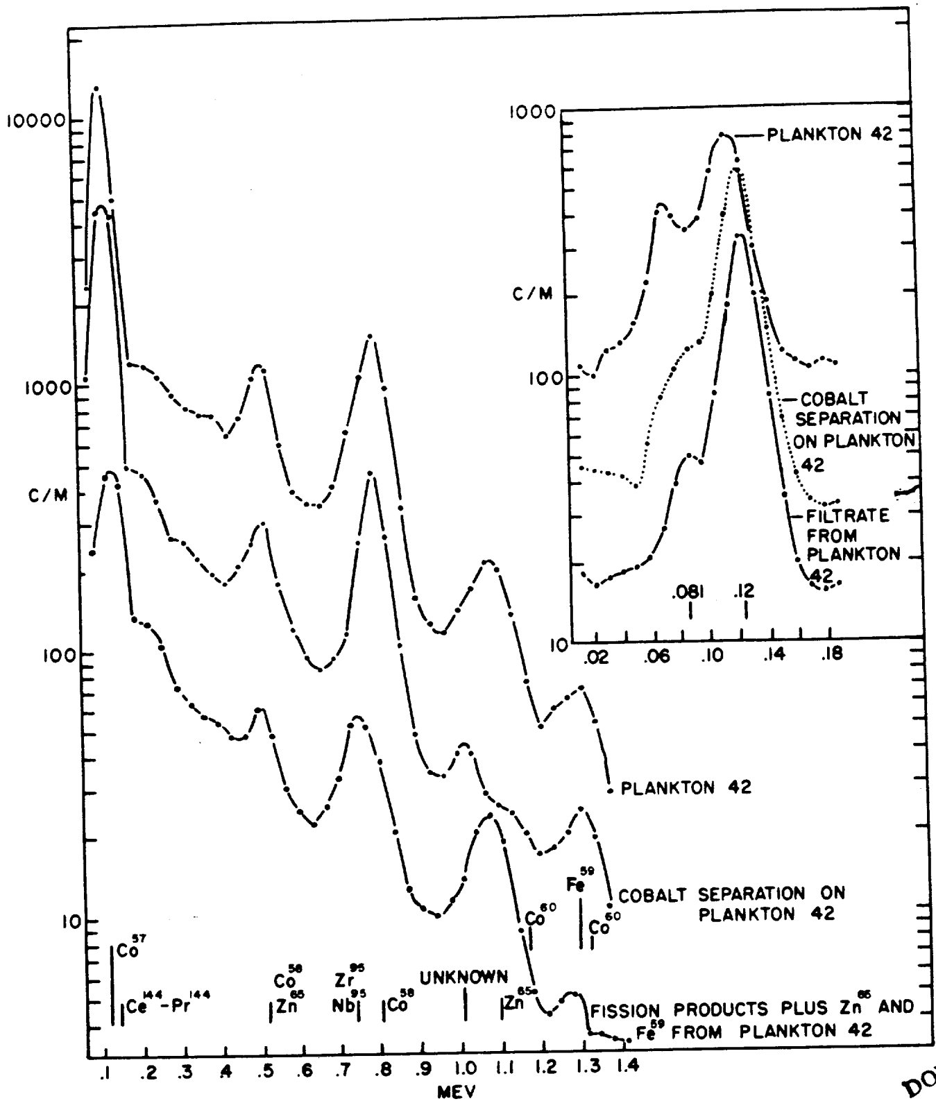
FIG. 12. Gamma spectra of Marsh plankton sample 42 and its chemically separated fractions.
