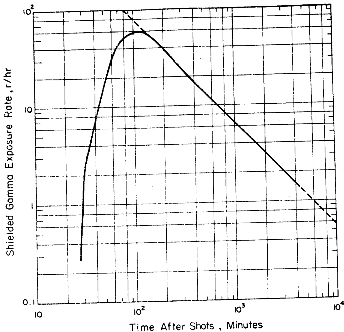
Figure 3.1 Residual exposure rate within blast shield versus time for Shot Zuni; Station 221.03, range 68,600 feet. For unshielded rate multiply by 1.4. Total 72.9-hour exposure, 502r.
