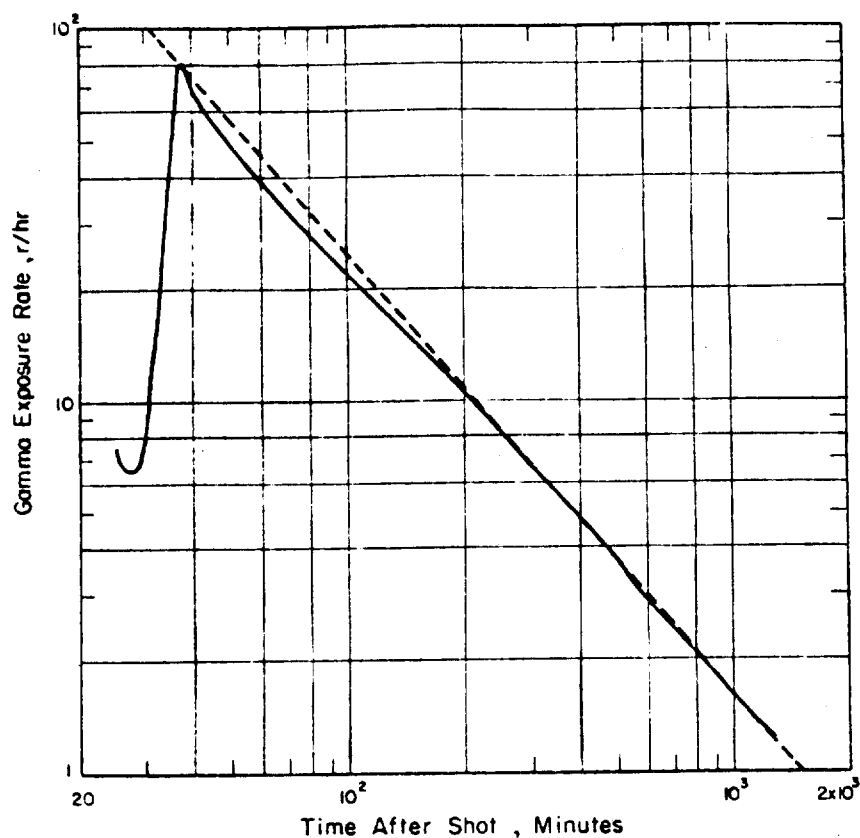
Figure 3.4 Unshielded residual exposure rate versus time for Shot Zuni; Station 221.02C, range 43,400 feet. Total 20.4-hour exposure, 125r.
