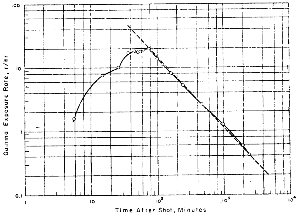
Figure 3.3 Residual exposure rate versus time for Shot Zuni; Station 221.01C, range 10,300 feet. For unshielded rate multiply by 1.4. Total 85-hour exposure, 99r.
