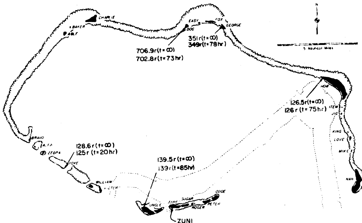
Figure 3.19 Map of Bikini Atoll showing unshielded residual exposures for Shot Zuni. This illustration gives exposures at Islands Dog, George, How, Uncle, and Yoke. See Table 3.1 for references to station designations, distances from ground zero, arrival times, and maximum exposure rates.
