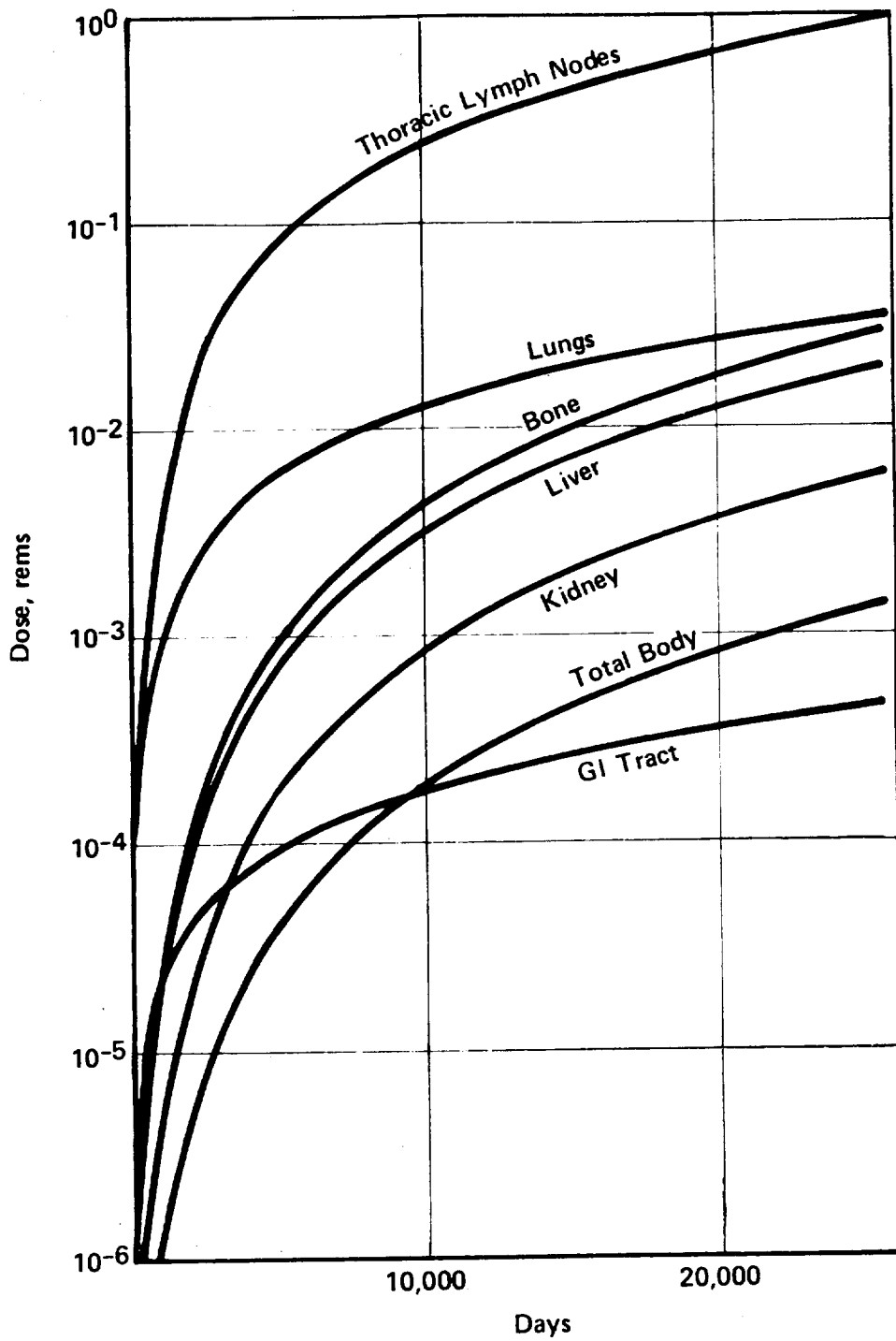
FIGURE 2. PREDICTED CUMULATIVE DOSES DUE TO 239 Pu IN DIFFERENT ORGANS OF STANDARD MAN
