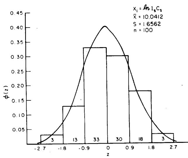
FIGURE 7. LOGNORMAL DISTRIBUTION OF PLUTONIUM UPTAKE FROM SOIL BY GRAZING CATTLE (Synthetic Composite Random Sample)
