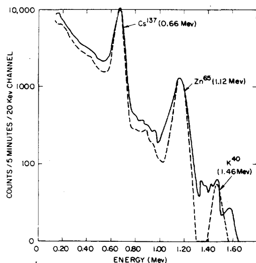
Figure 52. Gamma spectra of Marshallese male (subject #4, age 40, wt 70 kg - solid line) and normalized plastic phantom (containing 0.64 \mu\text{C} \text{Zn}^{65} , 1.22 \mu\text{C} \text{Cs}^{137} , and 140 g \text{K} - dashed line), 1959.
