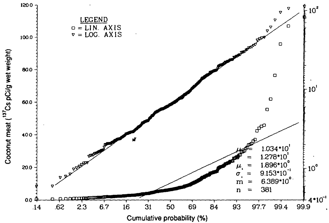
Figure 23. Probability plot of ^{137}\text{Cs} concentration in drinking-coconut meat on Eneu Island.
