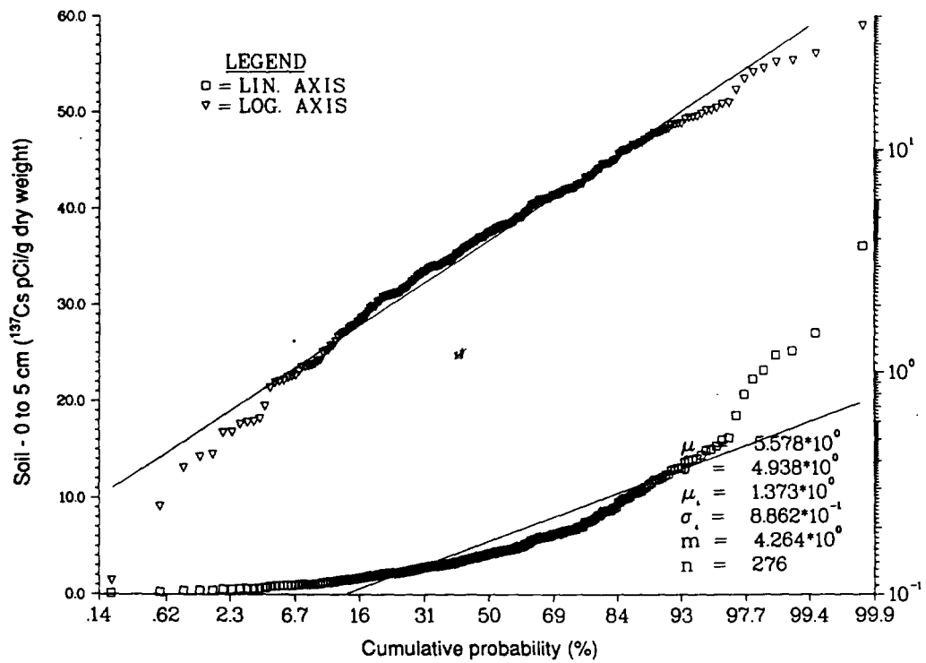
Figure 7. Probability plot of ^{137}\text{Cs} concentration in the top 0 to 5 cm of soil at Eneu Island.
