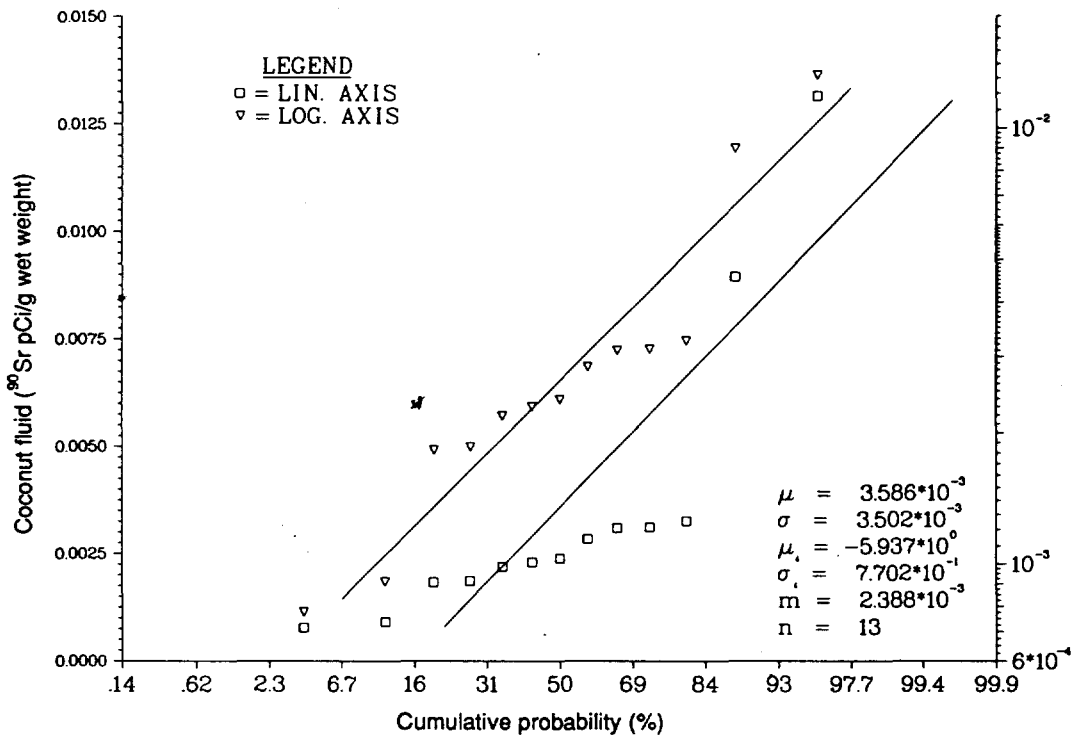
Figure 27. Probability plot of 90 Sr concentration in drinking-coconut fluid on Eneu Island.
