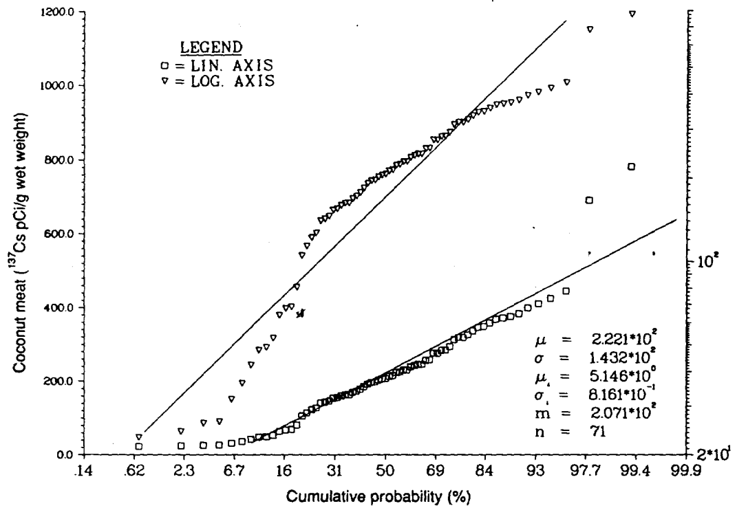
Figure 19. Probability plot of 137 Cs concentration in copra-coconut meat on Bikini Island.
