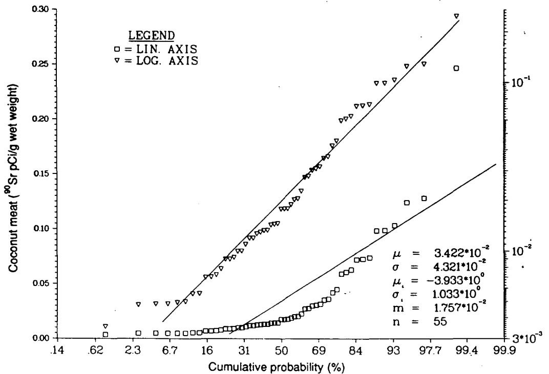
Figure 28. Probability plot of 90 Sr concentration in copra-coconut meat on Eneu Island.
