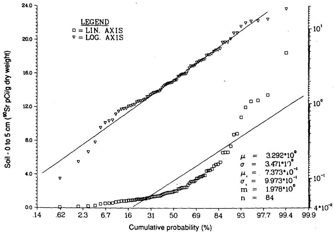
Figure 8. Probability plot of ^{90}\text{Sr} concentration in the top 0 to 5 cm of soil at Eneu Island.
