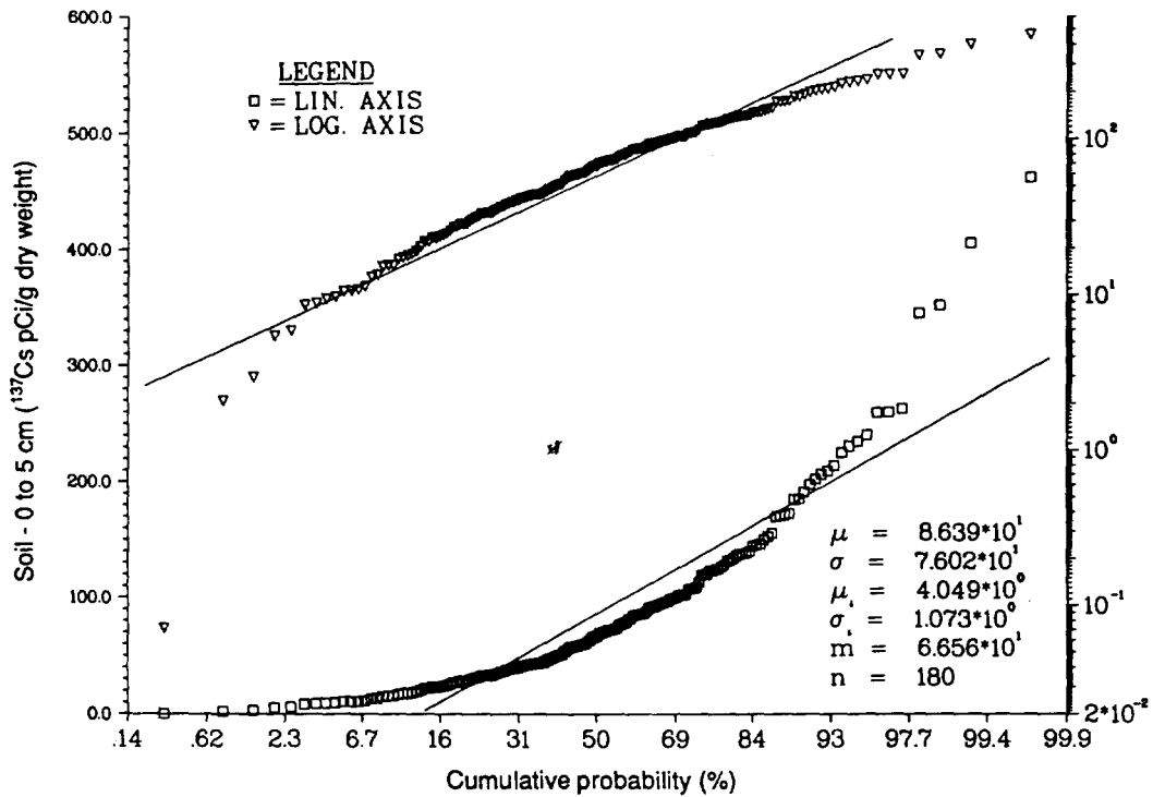
Figure 3. Probability plot of 137 Cs concentration in the top 0 to 5 cm of soil at Bikini Island.
