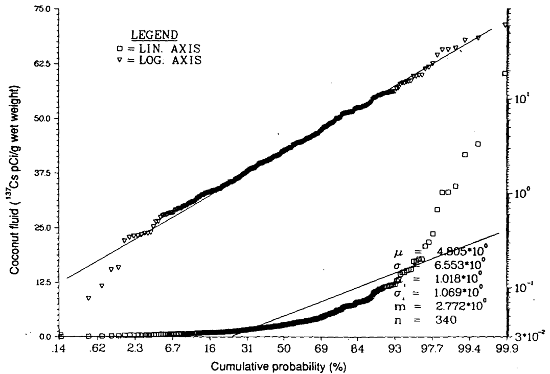
Figure 24. Probability plot of ^{137}\text{Cs} concentration in drinking-coconut fluid on Eneu Island.
