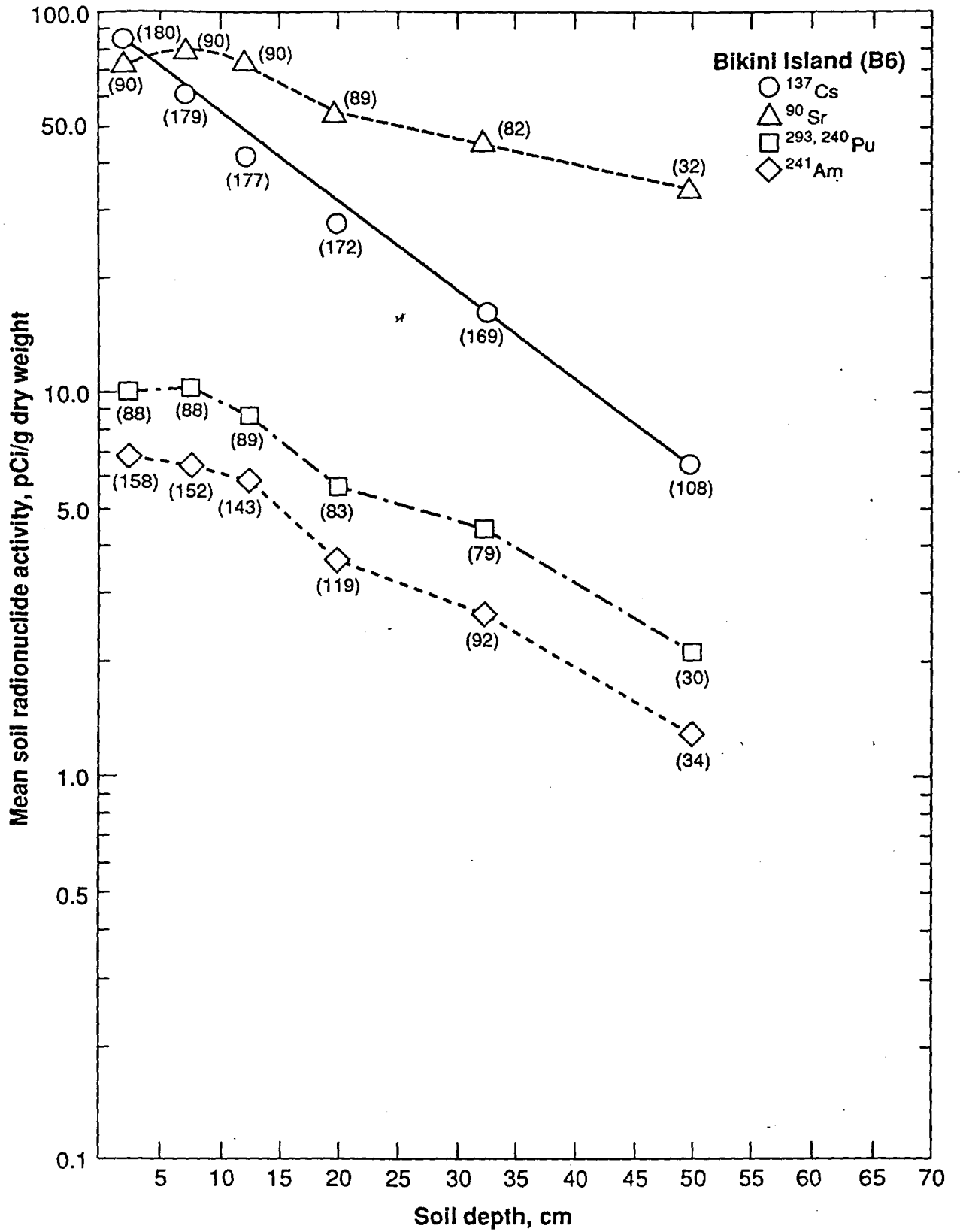
Figure 11. The mean value of ^{137}\text{Cs} , ^{90}\text{Sr} , ^{239+240}\text{Pu} , and ^{241}\text{Am} as a function of depth in the soil column at Bikini Island.
