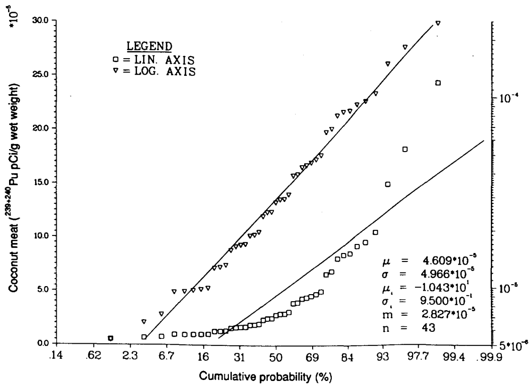
Figure 30. Probability plot of ^{239+240}\text{Pu} concentration in copra-coconut meat on Eneu Island.
