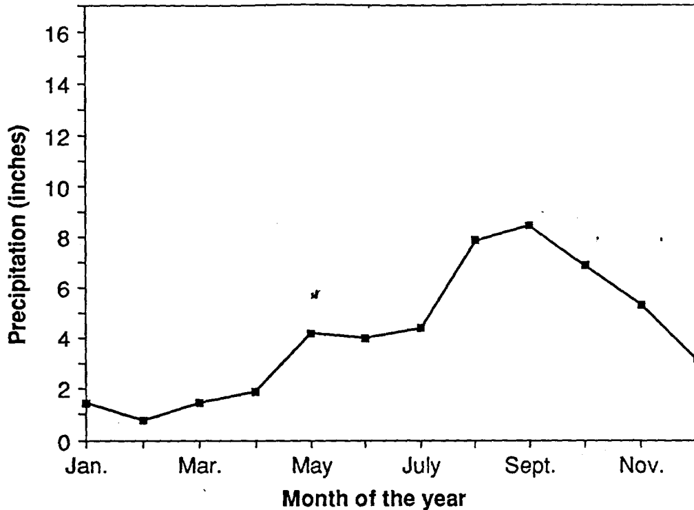
Figure 32. Average monthly rainfall at Bikini Atoll from 1982 through 1987.
