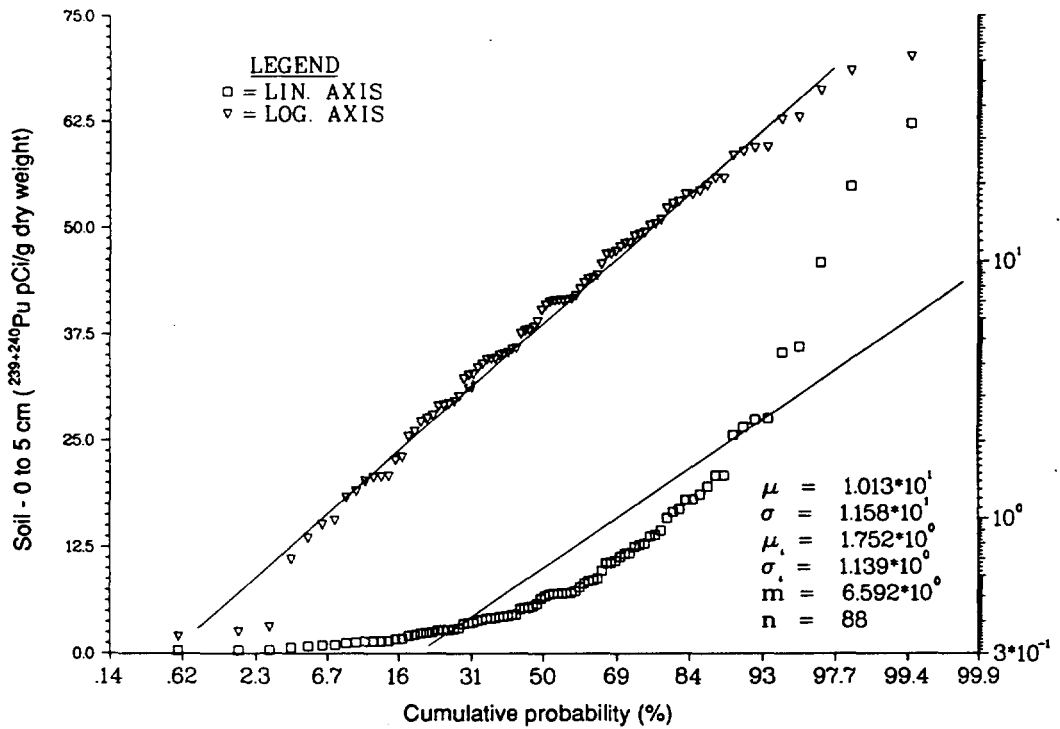
Figure 5. Probability plot of ^{239+240}\text{Pu} concentration in the top 0 to 5 cm of soil at Bikini Island.
