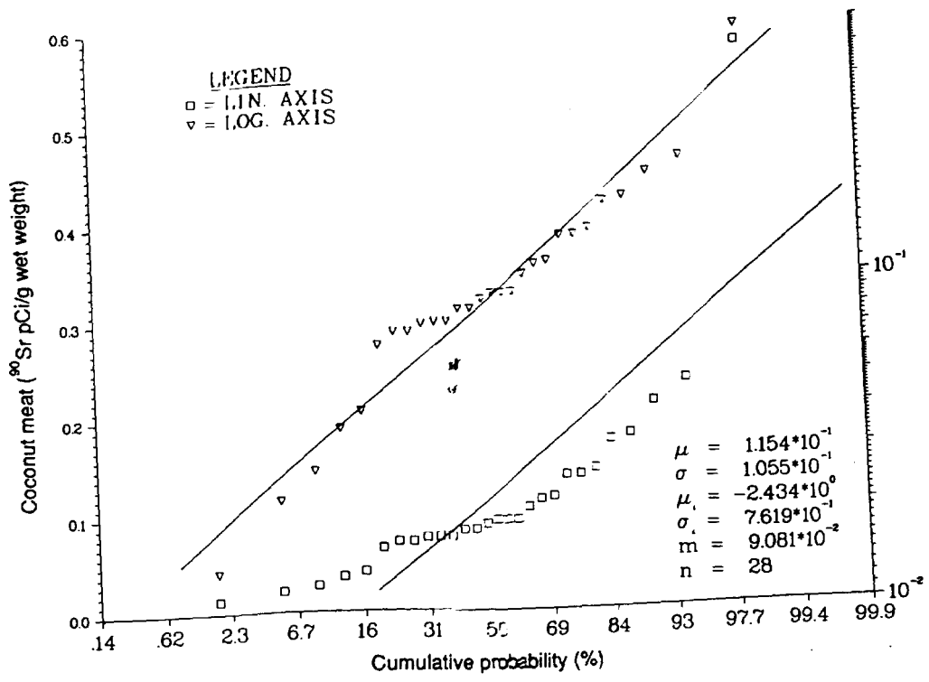
Figure 21. Probability plot of 90 Sr concentration in copra-coconut meat on Bikini Island.
