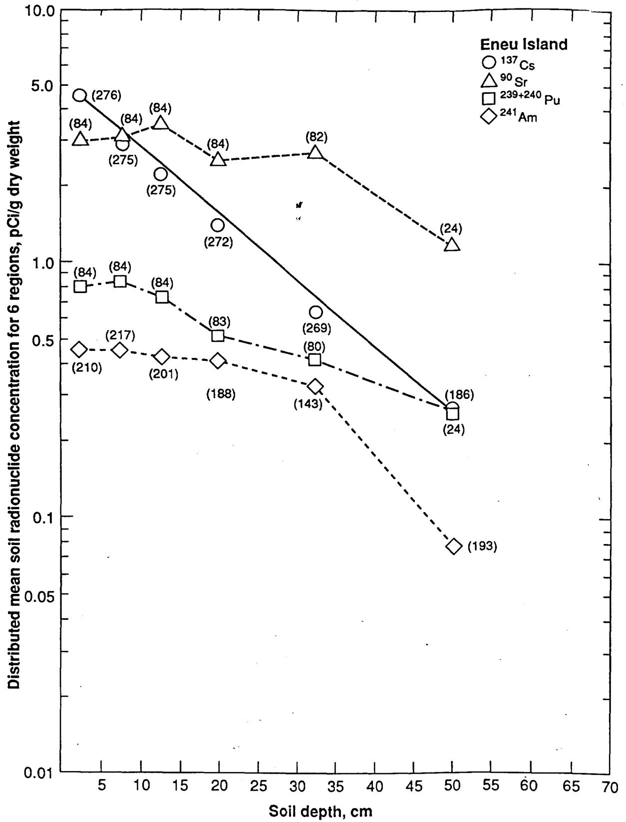
Figure 16. The distributed mean value of ^{137}\text{Cs} , ^{90}\text{Sr} , ^{239+240}\text{Pu} , and ^{241}\text{Am} as a function of depth in the soil column at Eneu Island.
