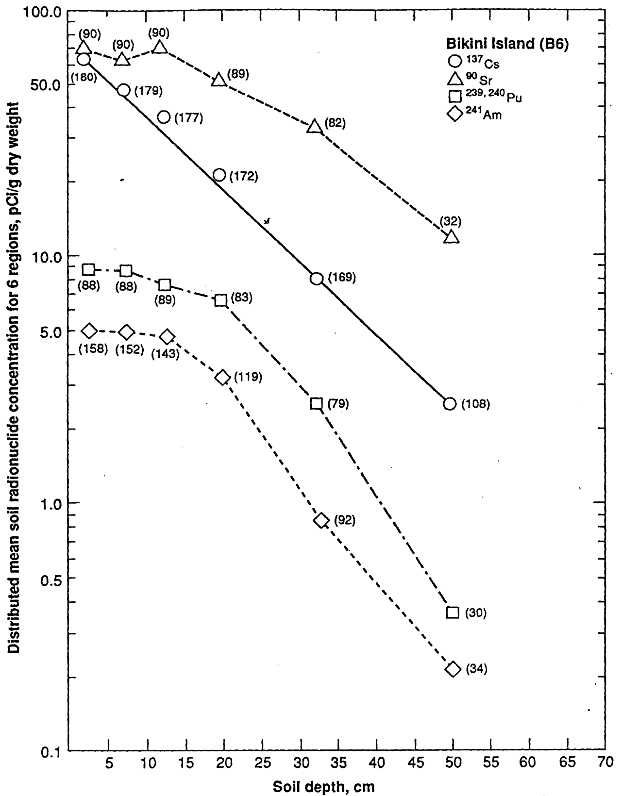
Figure 13. The distributed mean of ^{137}\text{Cs} , ^{90}\text{Sr} , ^{239+240}\text{Pu} , and ^{241}\text{Am} as a function of depth in the soil column at Bikini Island.
