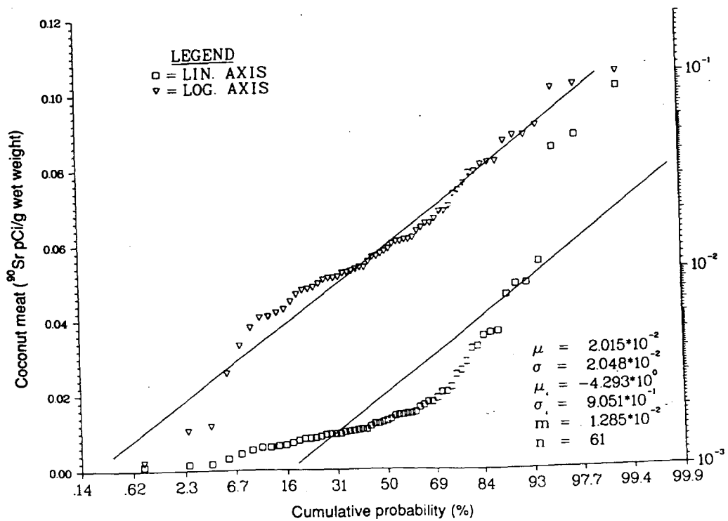
Figure 26. Probability plot of 90 Sr concentration in drinking-coconut meat on Eneu Island.
