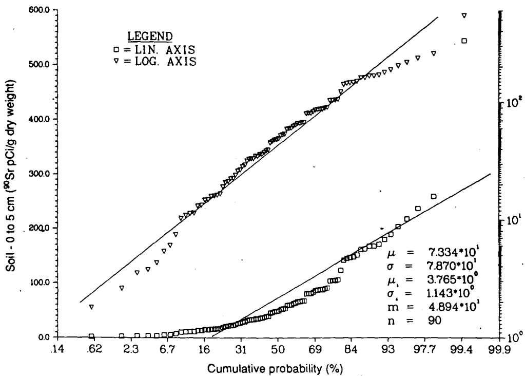
Figure 4. Probability plot of 90 Sr concentration in the top 0 to 5 cm of soil at Bikini Island.
