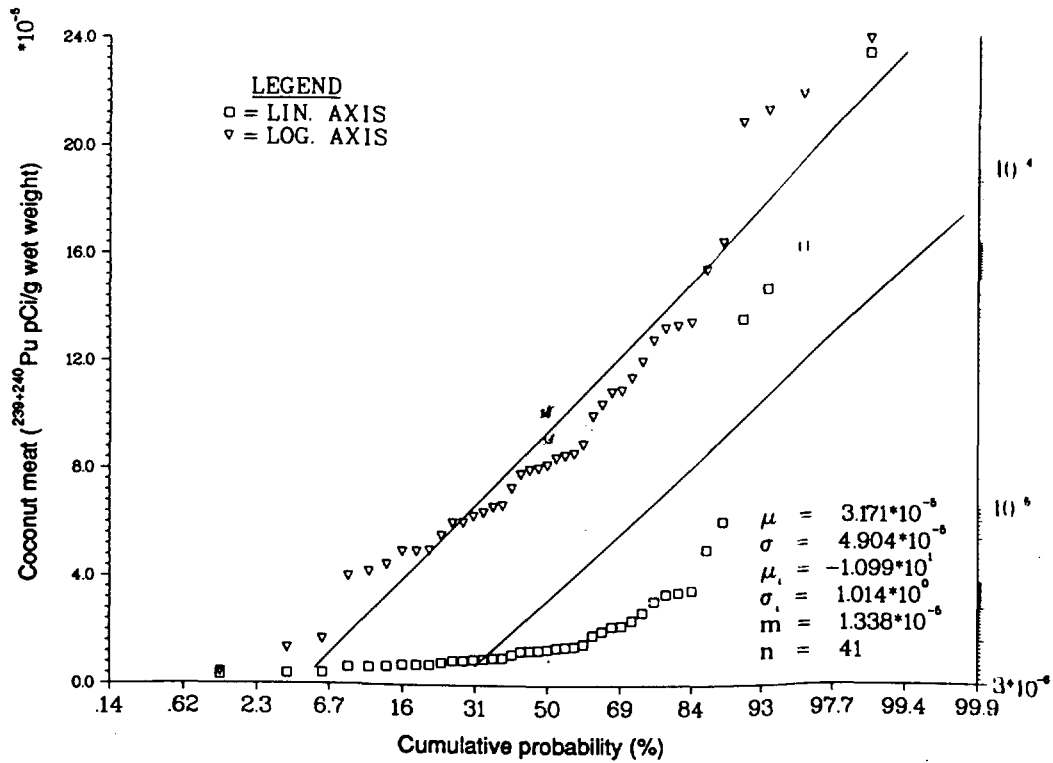
Figure 29. Probability plot of ^{239+240}\text{Pu} concentration in drinking-coconut meat on Eneu Island.
