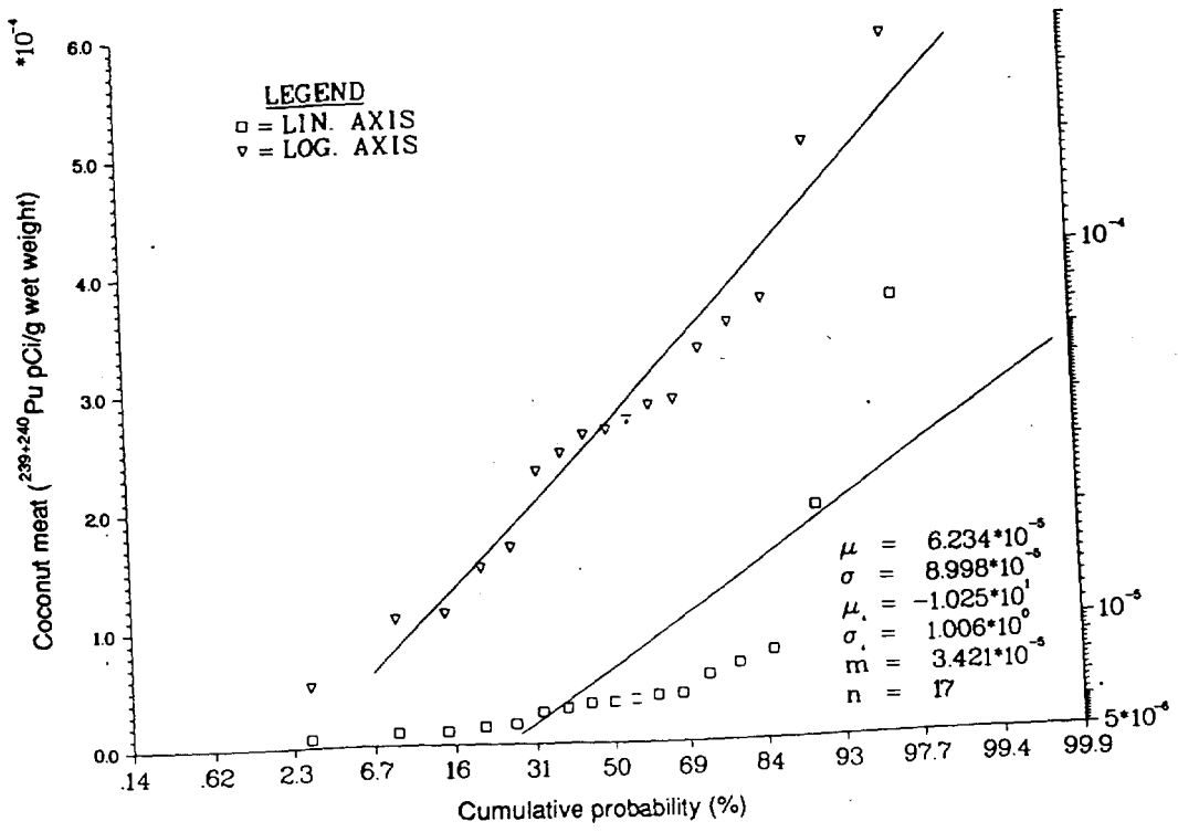
Figure 22. Probability plot of 239+240 Pu concentration in drinking-coconut meat on Bikini Island.
