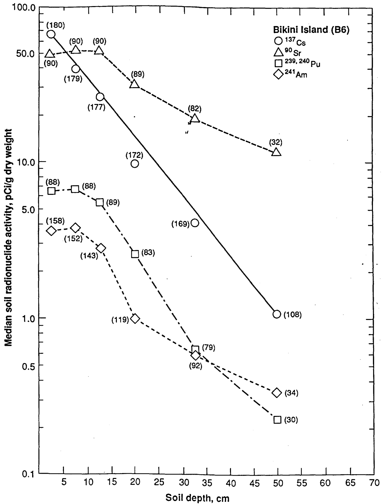
Figure 12. The median value of ^{137}\text{Cs} , ^{90}\text{Sr} , ^{239+240}\text{Pu} , and ^{241}\text{Am} as a function of depth in the soil column at Bikini Island.
