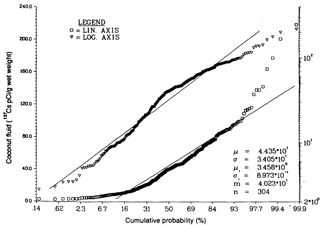
Figure 18. Probability plot of ^{137}\text{Cs} concentration in drinking-coconut fluid on Bikini Island.
