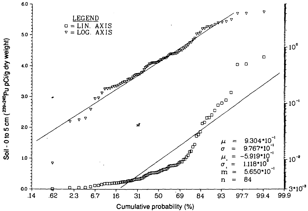
Figure 9. Probability plot of ^{239+240}\text{Pu} concentration in the top 0 to 5 cm of soil at Eneu Island.
