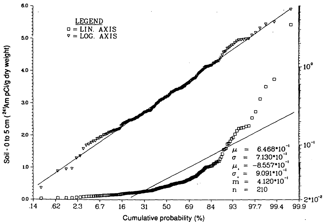
Figure 10. Probability plot of ^{241}\text{Am} concentration in the top 0 to 5 cm of soil at Eneu Island.
