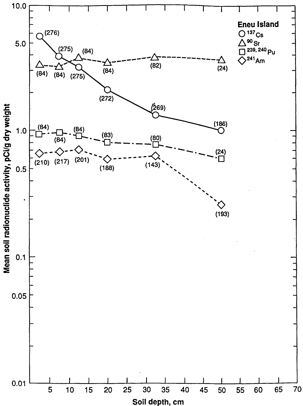
Figure 14. The mean value of ^{137}\text{Cs} , ^{90}\text{Sr} , ^{239+240}\text{Pu} , and ^{241}\text{Am} as a function of depth in the soil column at Eneu Island.
