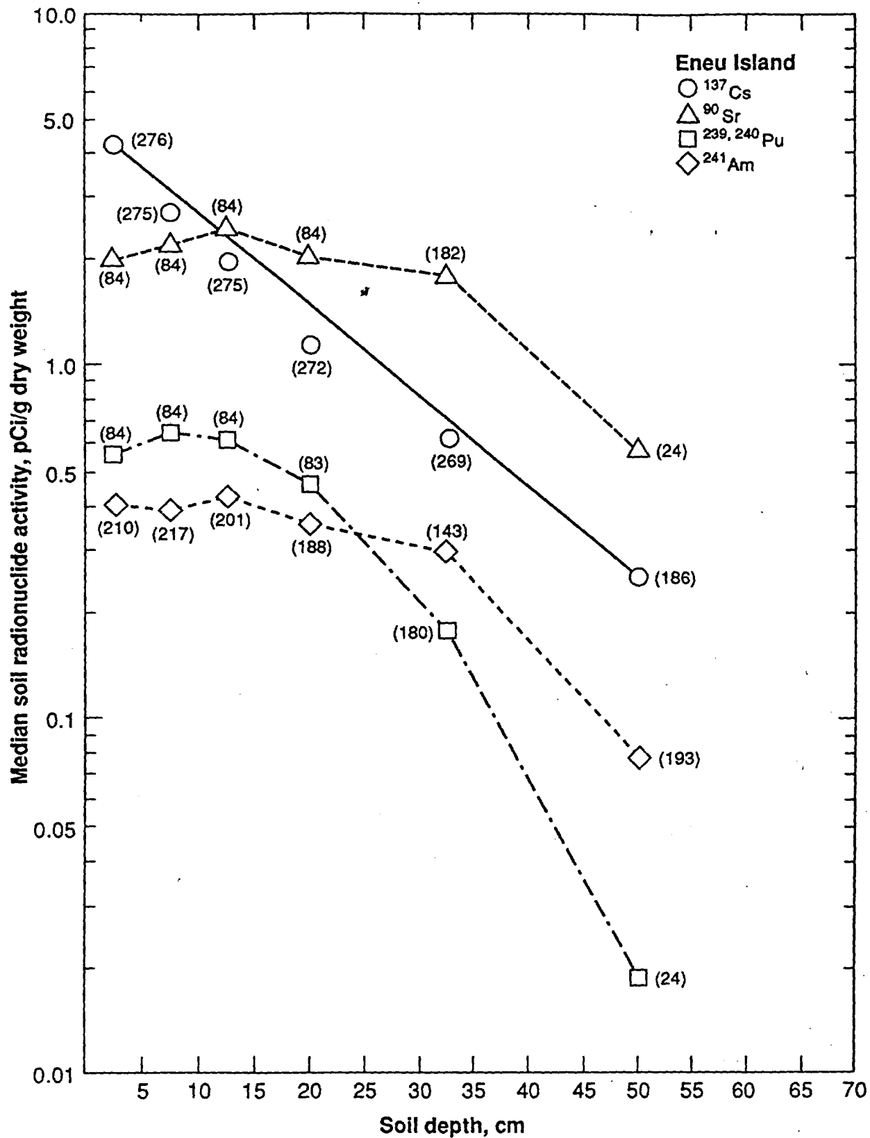
Figure 15. The median value of ^{137}\text{Cs} , ^{90}\text{Sr} , ^{239+240}\text{Pu} , and ^{241}\text{Am} as a function of depth in the soil column at Eneu Island.
