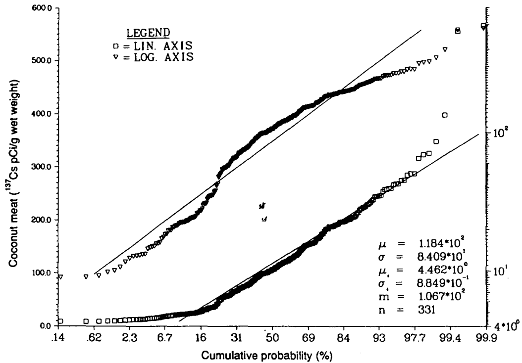
Figure 17. Probability plot of ^{137}\text{Cs} concentration in drinking-coconut meat on Bikini Island.
