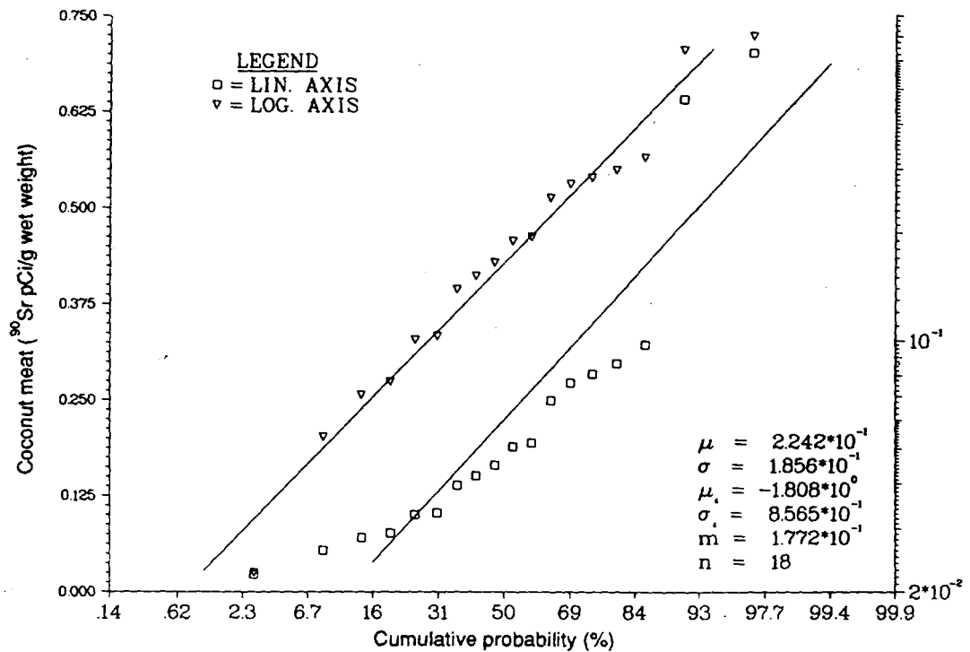
Figure 20. Probability plot of 90 Sr concentration in drinking-coconut meat on Bikini Island.
