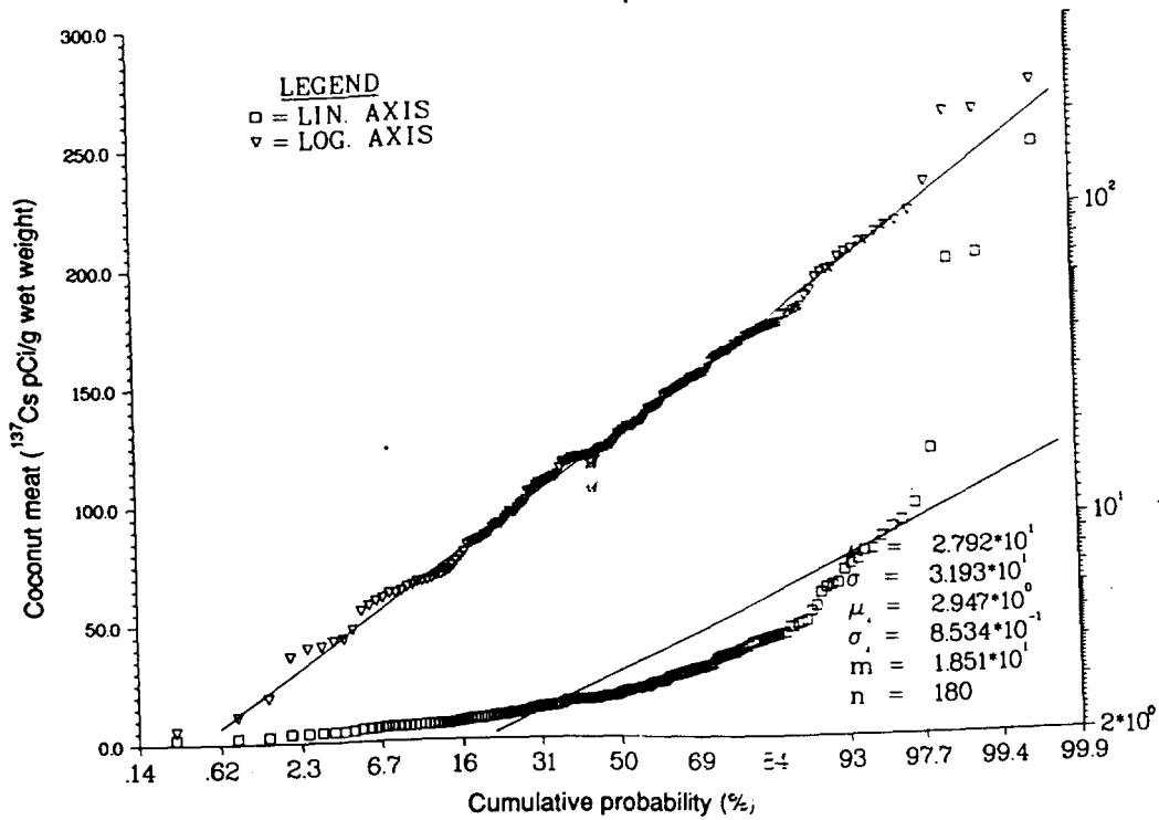
Figure 25. Probability plot of 137 Cs concentration in copra-coconut meat on Eneu Island.
