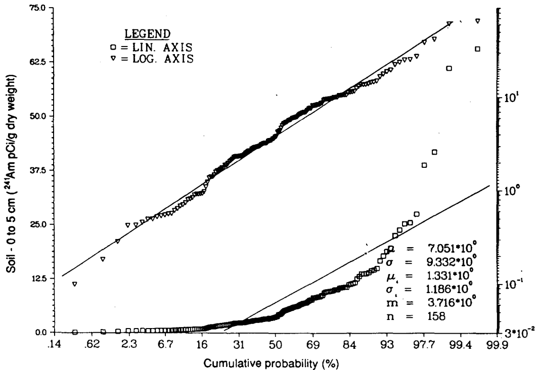
Figure 6. Probability plot of ^{241}\text{Am} concentration in the top 0 to 5 cm of soil at Bikini Island.
