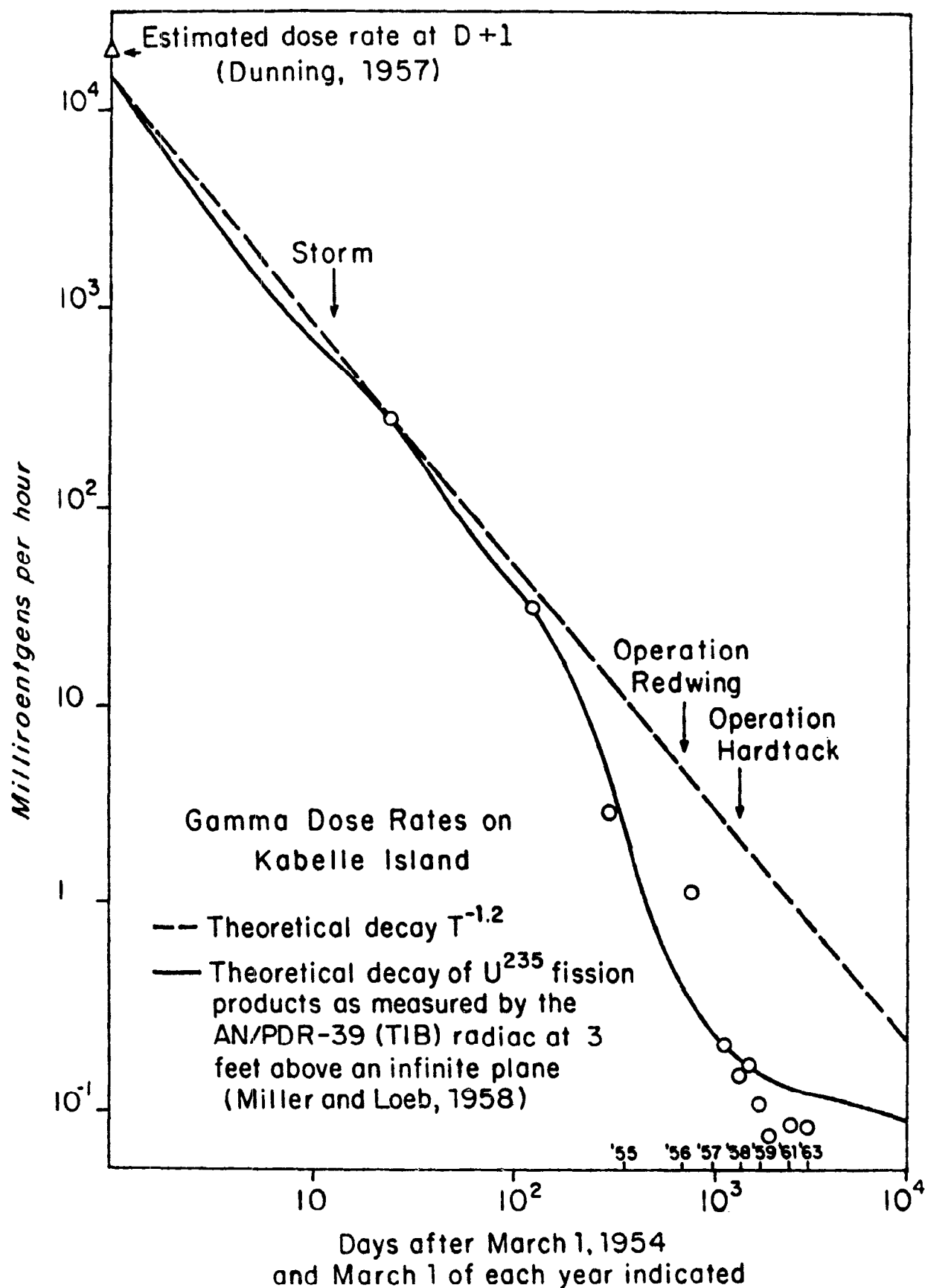
Fig. 3. Decline of Gamma Dose Rates at Kaballe Islet.
