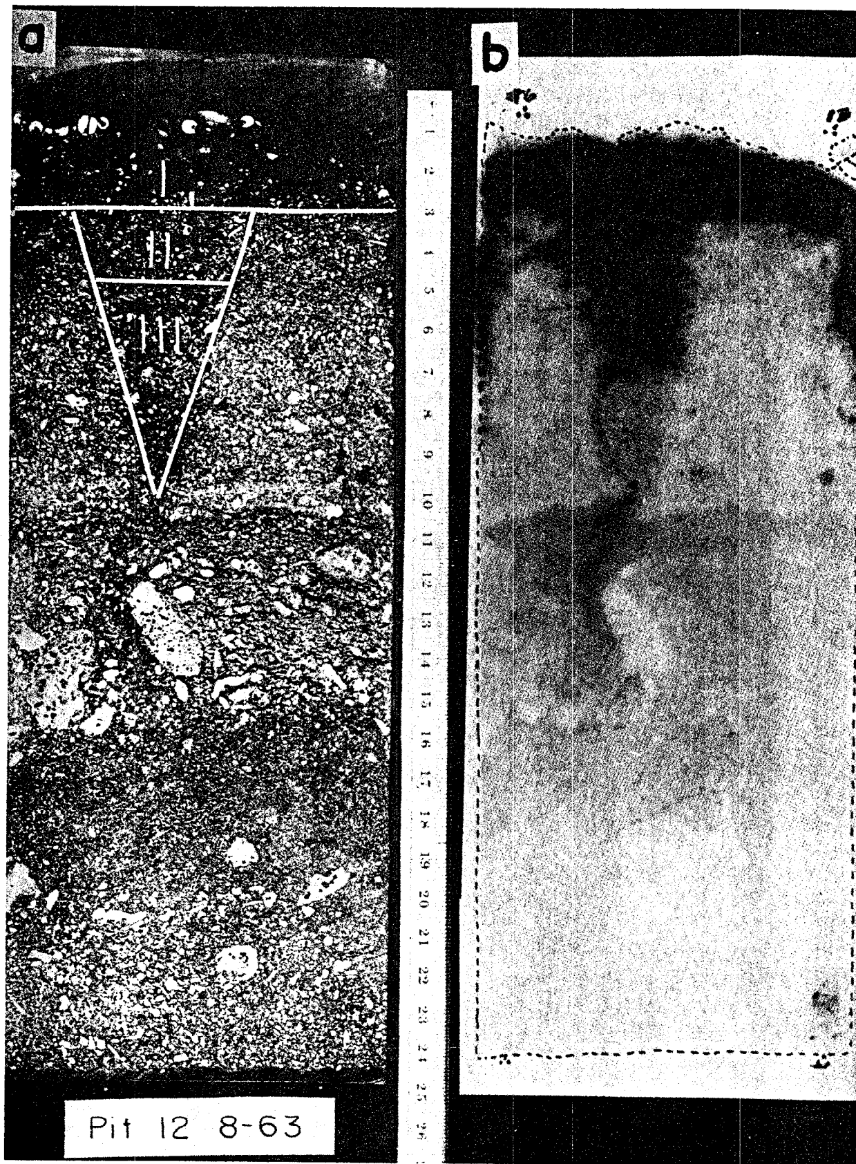
Fig. 14. Photograph and radioautograph of old soil showing correspondence of radioactive portions to organic matter.
