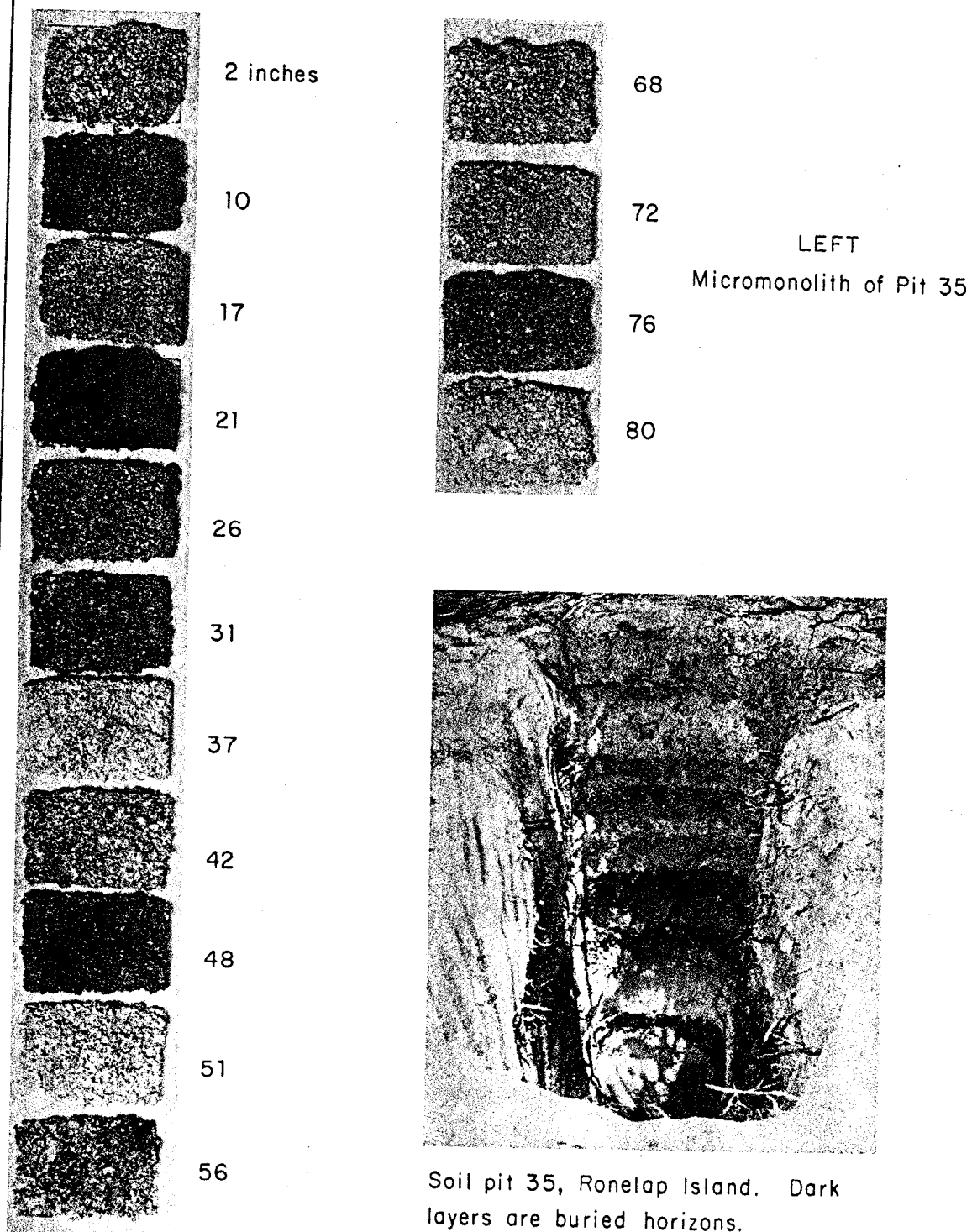
Fig. 1. Beach Ridge Sand, Rongelap Island. This soil type occurs on the island beach ridges. The pit shown above is seven feet deep and contains six buried horizons.
