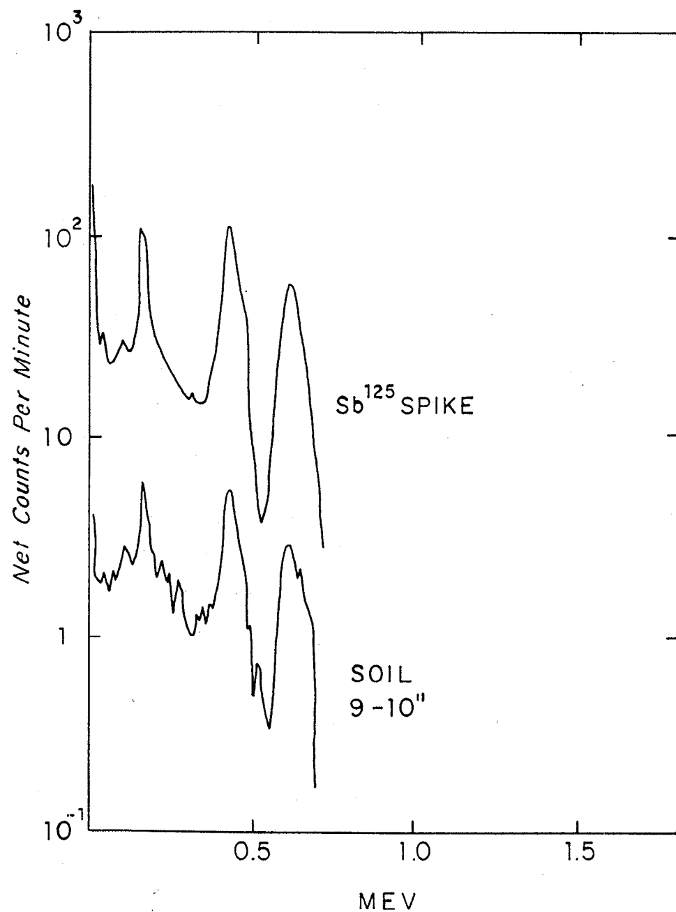
Fig. 10. Gamma-ray spectrum of young soil from a depth increment of 9 to 10 inches compared with the gamma spectrum of \text{Sb}^{125} .
