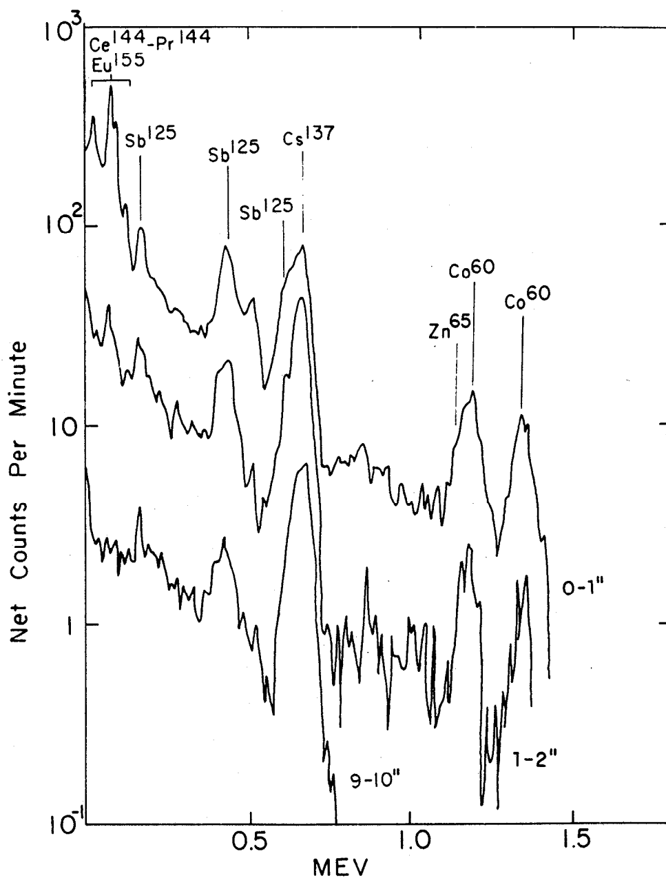
Fig. 5. Gamma-ray spectra of equal amounts of old soil from different depths.
