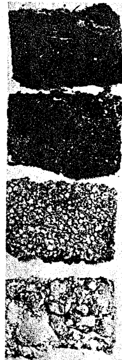
Micromonolith of Pit 38
