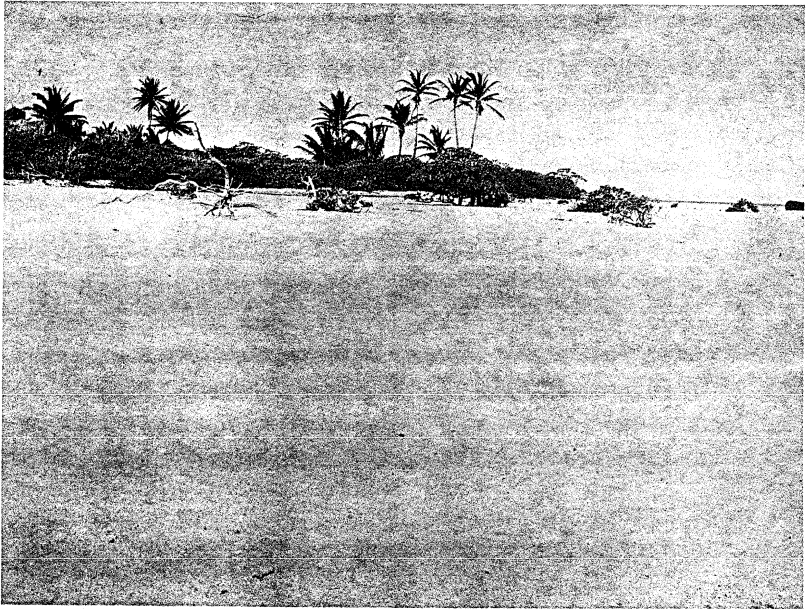
Fig. 13. An area of young soil subject to erosion.
