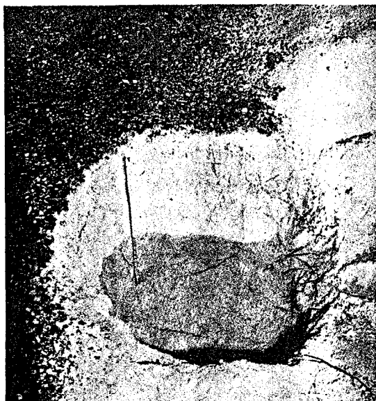
Soil pit 6. Black areas are crusts formed by algae.
