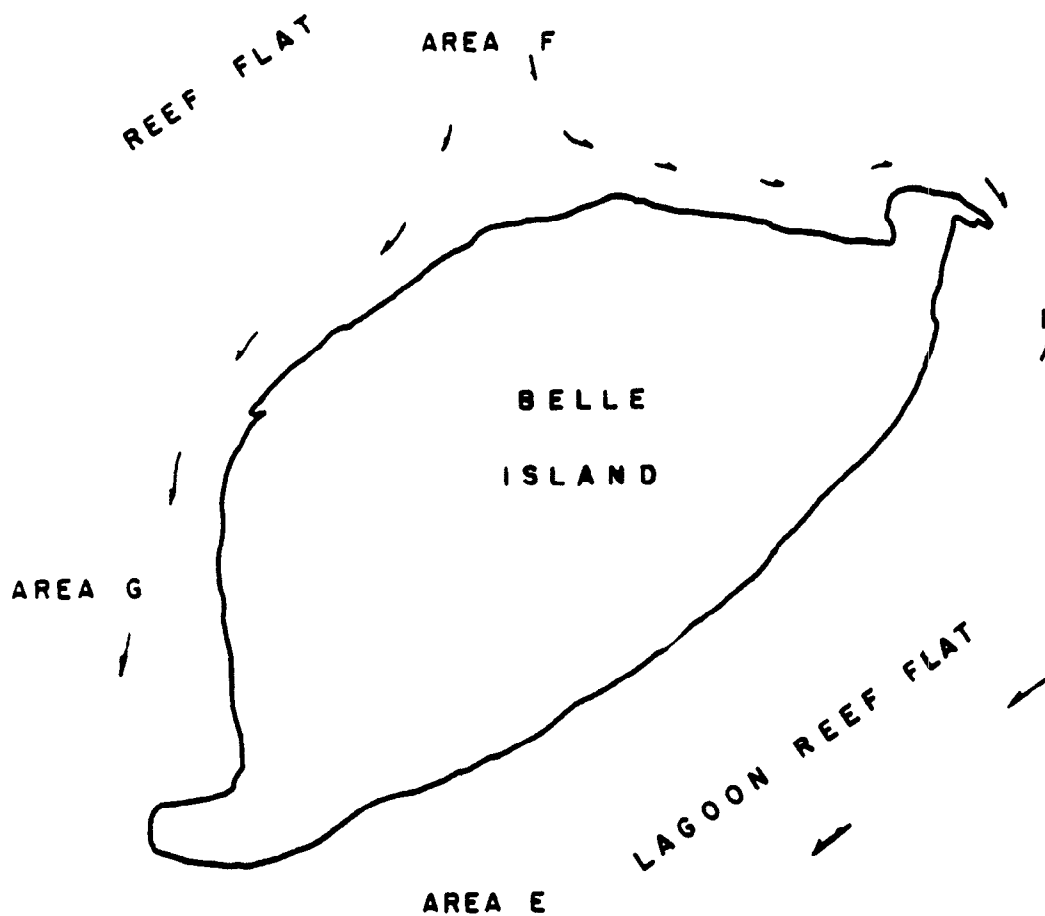
Fig. 1. Map of the north reef and islands of Eniwetok Atoll (top) with an enlarged map of Belle Island (bottom) showing typical current patterns. The wind rose indicates prevailing winds.
